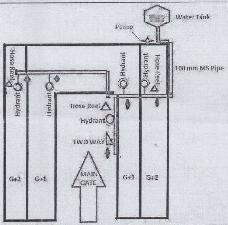
FIRE HYDRANT SYSTEM DRAWING, MOTHER PRIDE SCHOOL DHEMAJI
